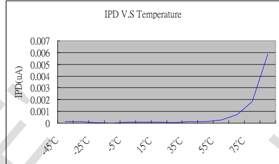
Power-Down Current
