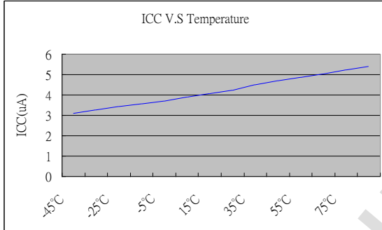
Supply Current
