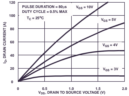
Figure 6. Saturation Characteristics
